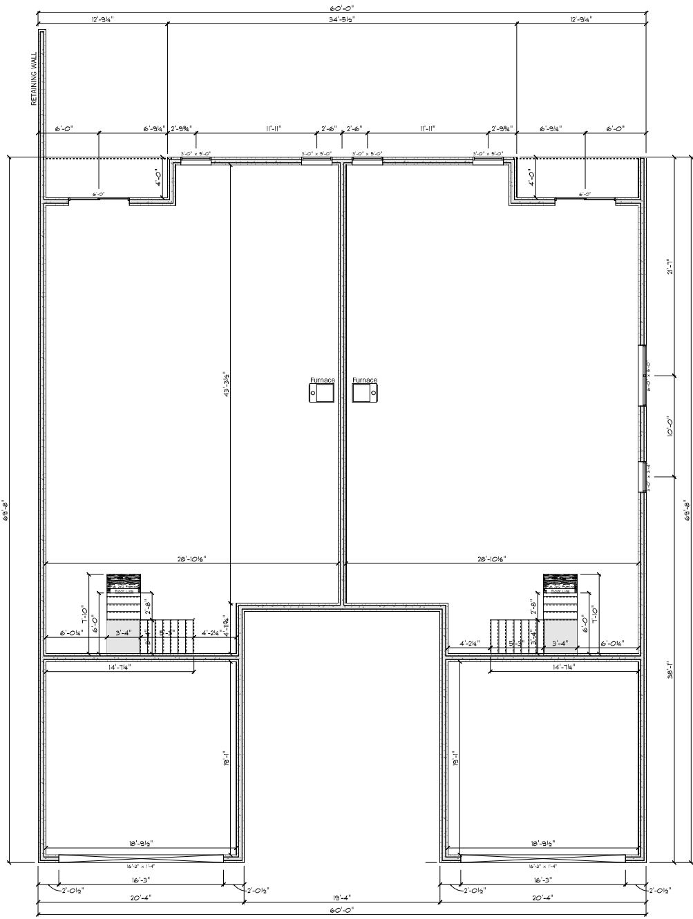
MAIN FLOOR PLAN 1/4" = 1'
