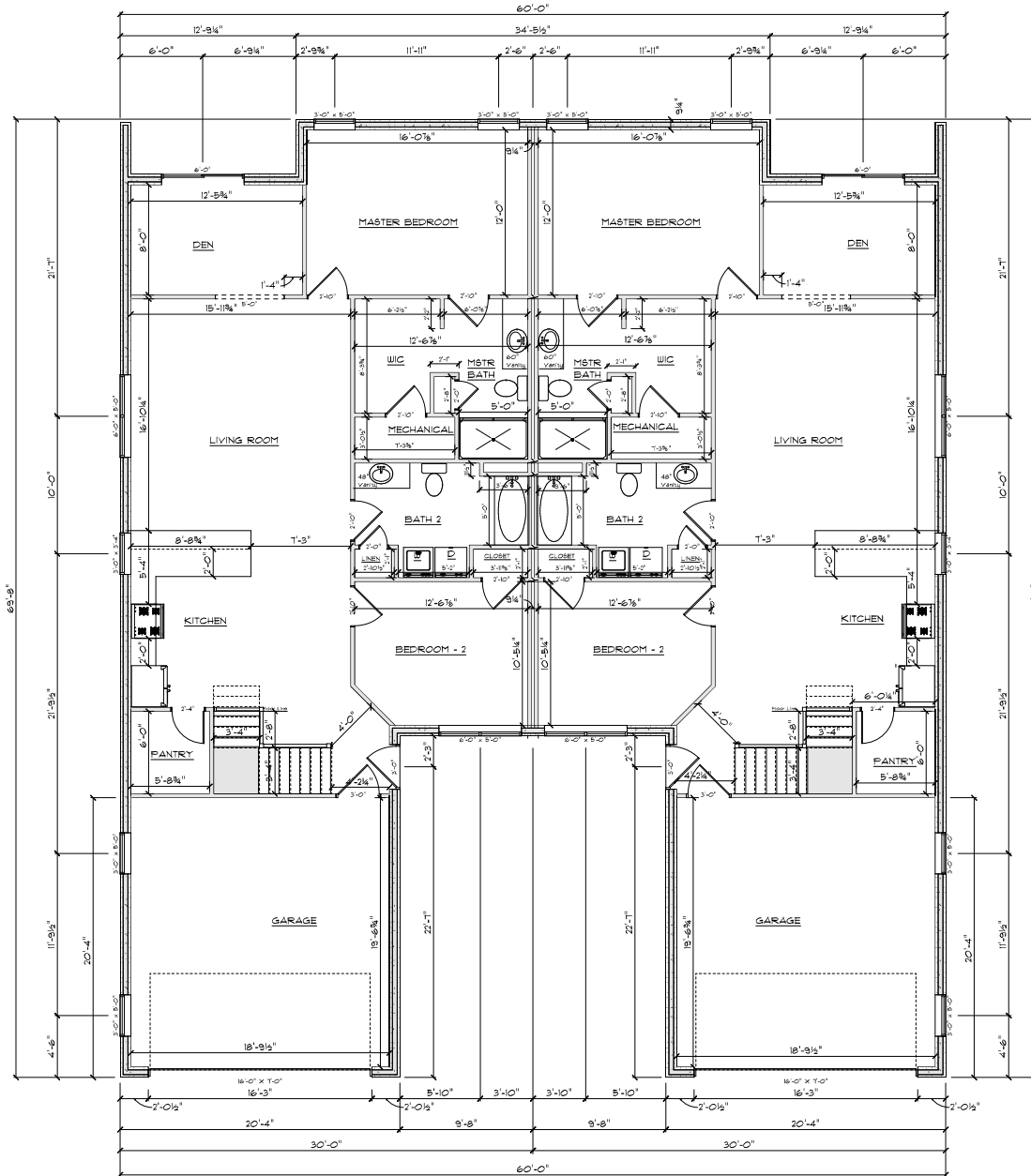
MAIN FLOOR PLAN 1/4" = 1'
